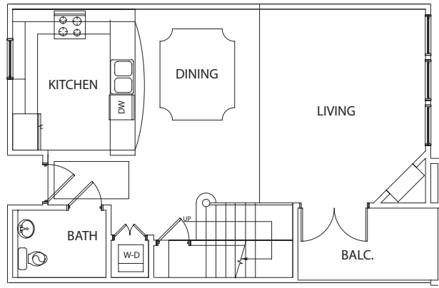
FIRST FLOOR PLAN TYPE "P"
